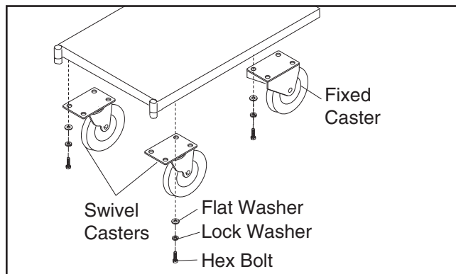
Figure 2. Installing casters.
